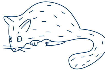
LOIR
